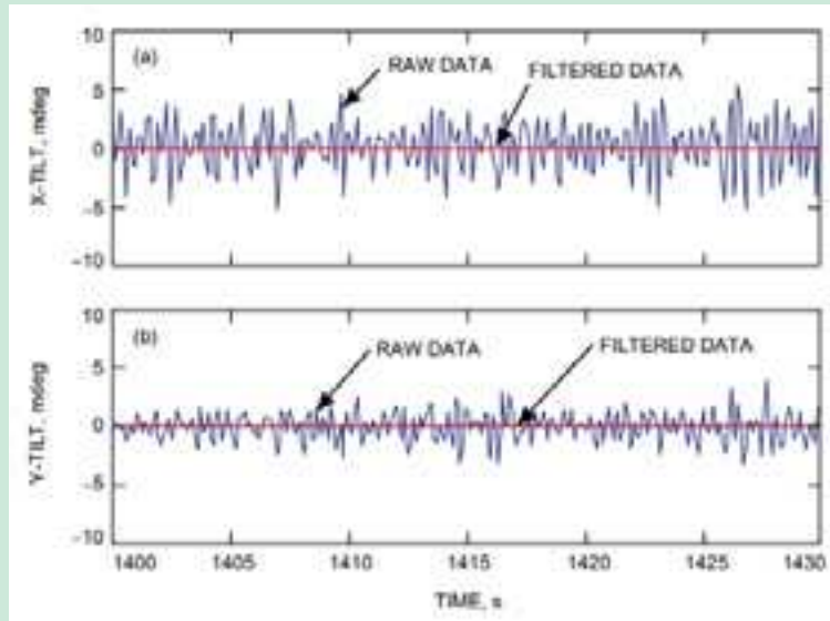
Figure 4. A sample of the tilt measurements of the ME tower collected at a 1G-Hz sampling rate during tracking: (a) x-tilts and (b) y-tilts.
