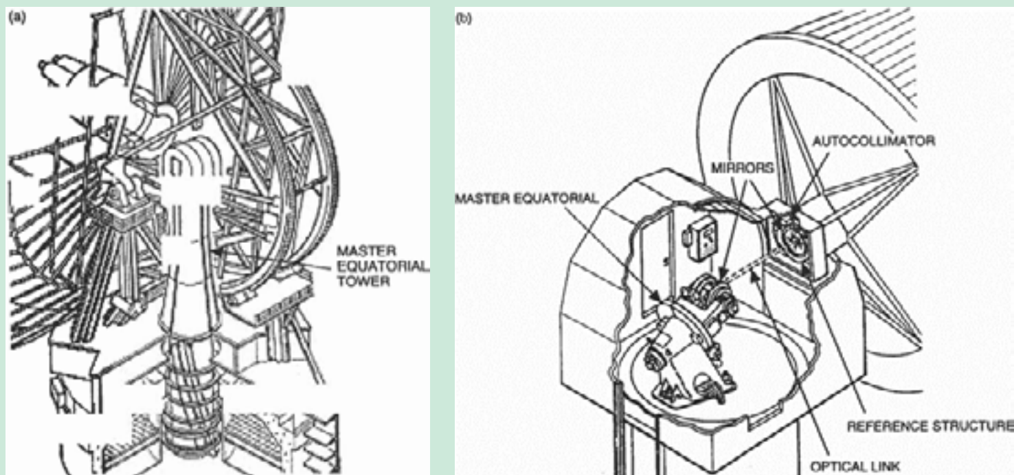
Figure 1. Antenna and ME tower cross-sections: (a) the ME tower and (b) the ME, autocollimator, and mirrors.
