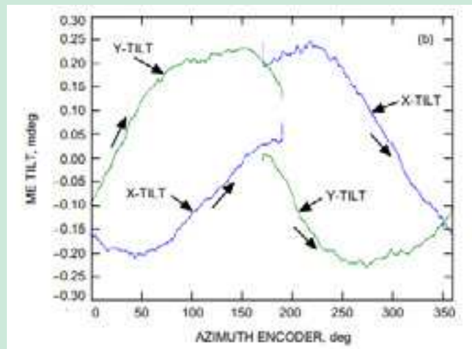
Figure 10. Slow-varying ME tower tilts during antenna slew: (a) counterclockwise slew and (b) clockwise slew.
