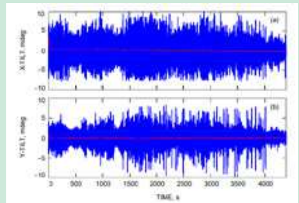
Figure 3. Tilts of the ME tower collected at a 1().Hz sampling rate during tracking: (a) x-UHS and (b) y-tilts.
