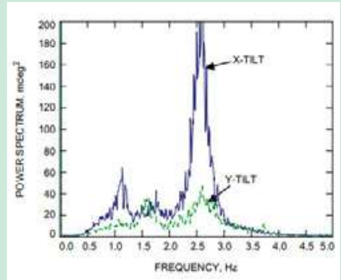
Fig. 5. The power spectrum of the x- and y-tilt data during tracking.
