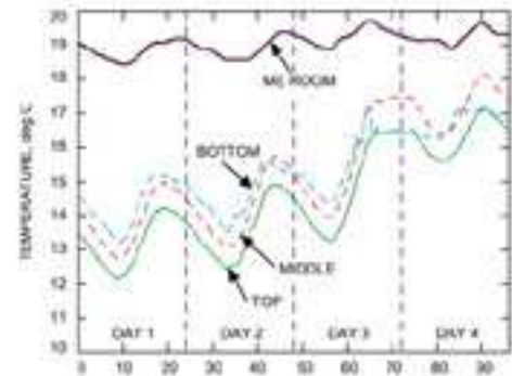
Figure 16. Temperature in the ME room and the ME tower
