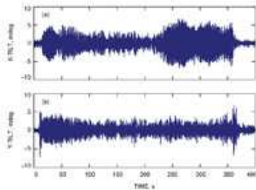
Figure 6. The ME tower tilts during elevation slew: (a) x-tilt and (b) y-tilt.
