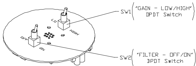
BOTTOM VIEW (Solder/Switch Side)
