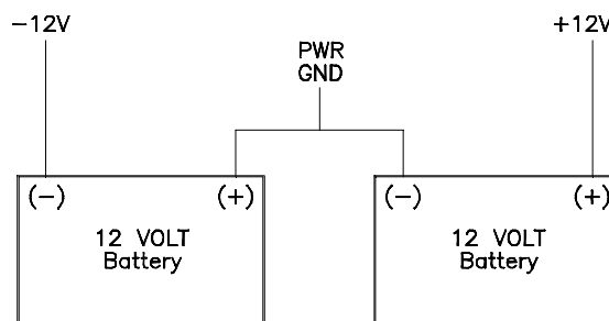
Figure 4 - Power Supply Connections for Model 83162
