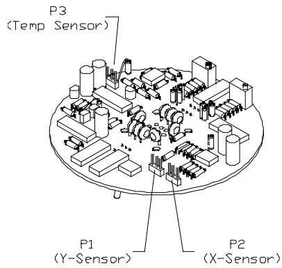
TOP VIEW (Component Side)
