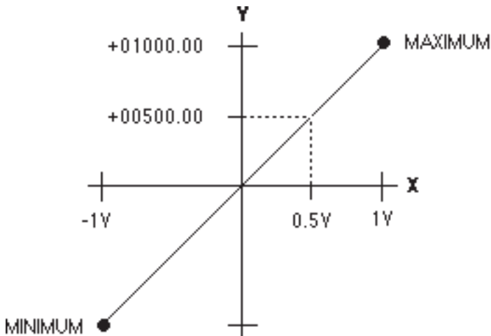
Figure 5. Function Endpoints
