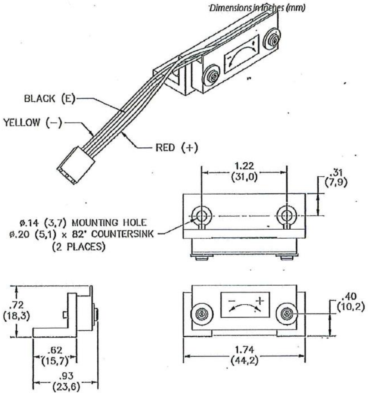
84053 OUTLINE DRAWING
