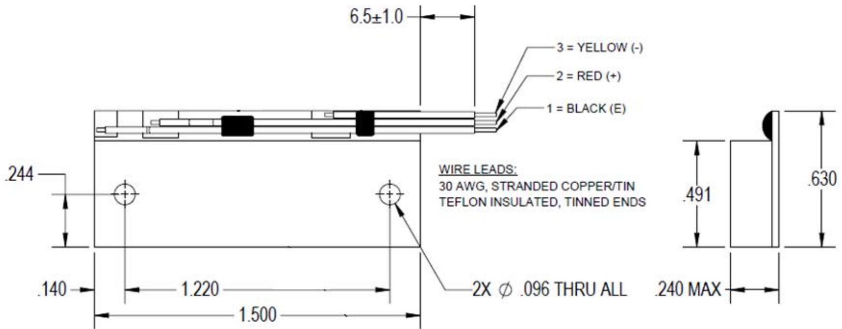
59577 OUTLINE DRAWING
